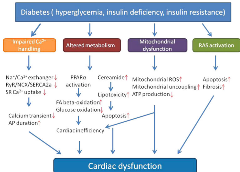
Fig. 1 Proposed mechanism of impaired cardiac function in diabetes. RyR ryanodine receptor, NCX sodium/calcium exchanger, SERCA2a sarcoplasmic reticulum \text{Ca}^{2+} -ATPase 2a, SR sarcoplasmic reticulum, AP action potential, PPAR \alpha peroxisome proliferator-activated receptor alpha, FA fatty acid, ROS reactive oxygen species
